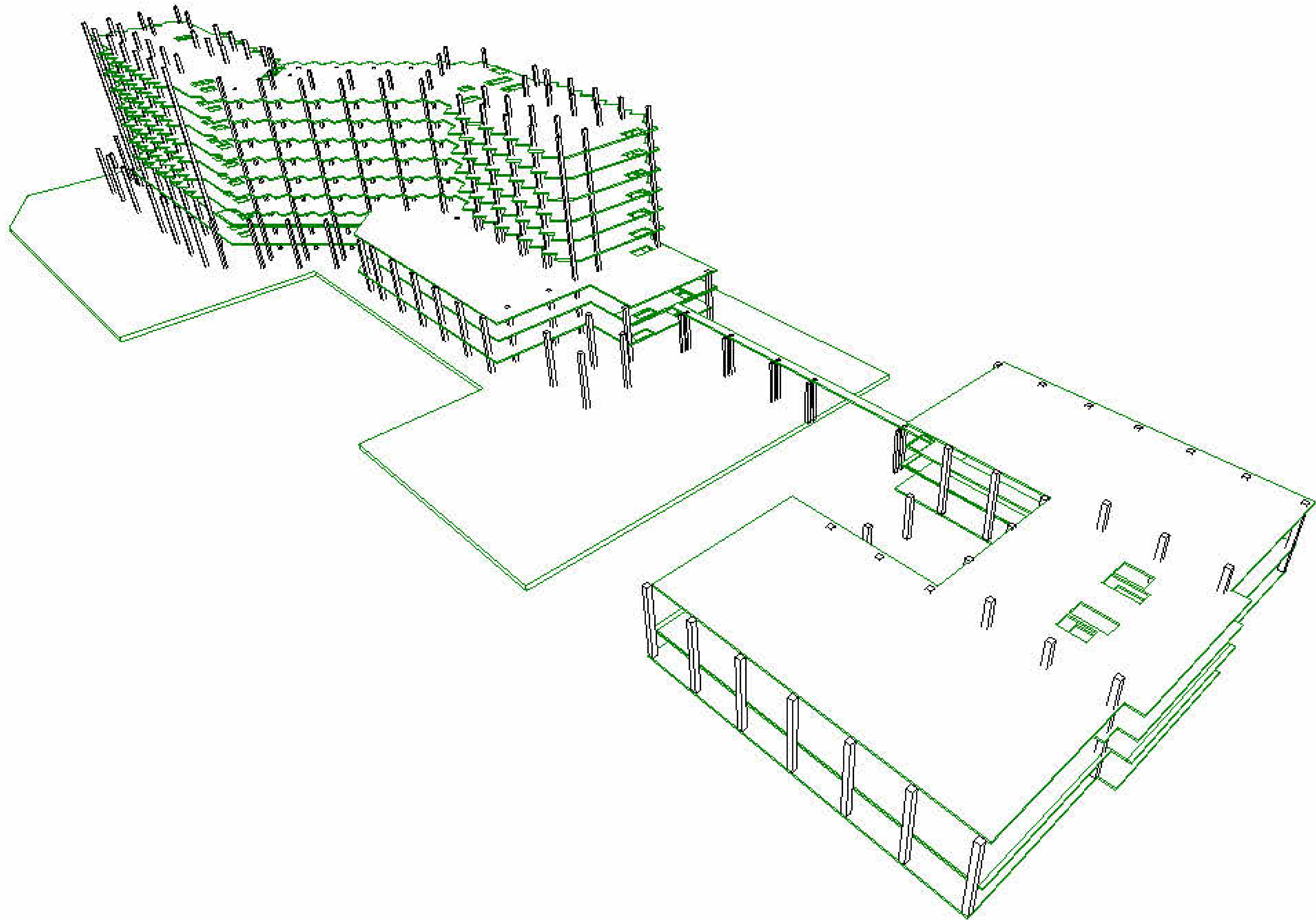
1 STRUCTURAL PERSPECTIVE 2 A-21 NOT TO SCALE
