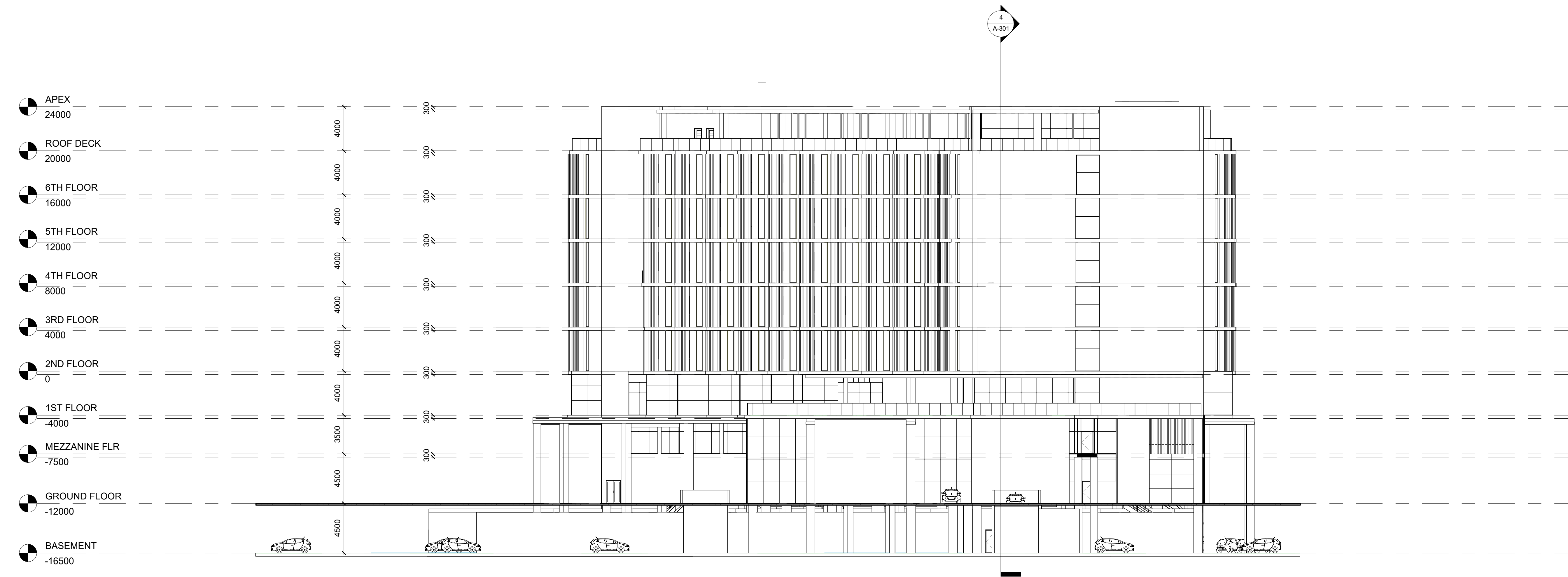
2 A-202 HOTEL RIGHT VIEW ELEVATION 1 : 200
