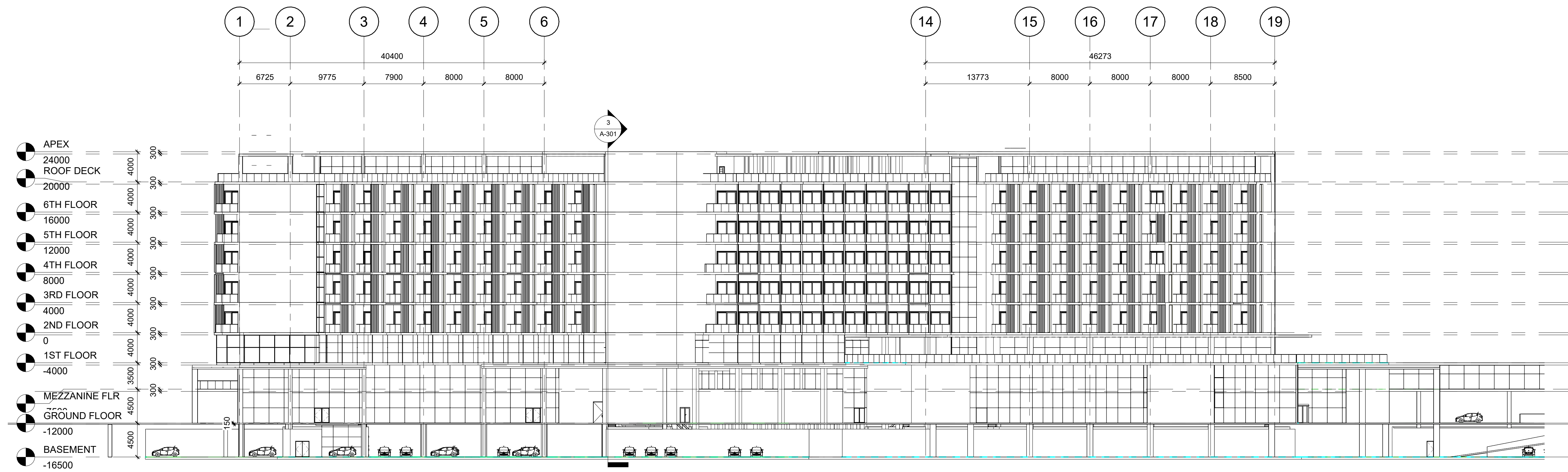
1 HOTEL FRONT VIEW ELEVATION A-201 1 : 300
